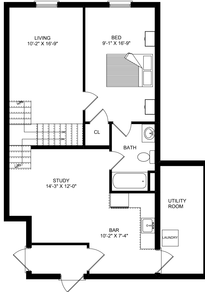
GARDEN LEVEL FLOOR PLAN 985 SQ FT
