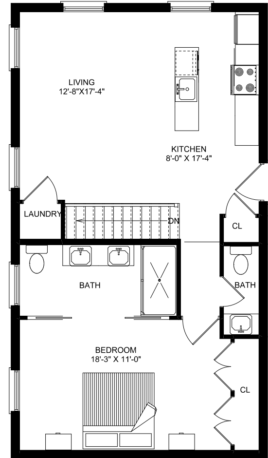
FIRST FLOOR PLAN 825 SQ FT
